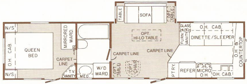
35' ST. PAUL AXLE WT. 8285 HITCH WT. 950
