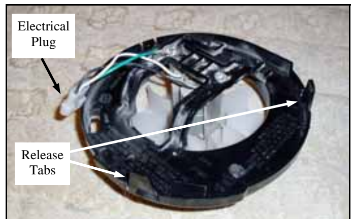
Fan motor assembly is removed by unplugging and pulling on release tabs.
